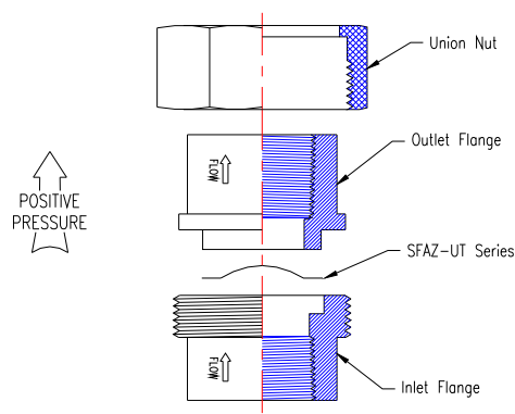
Figure 2 – Flat Seated Disk Union Type Holder
