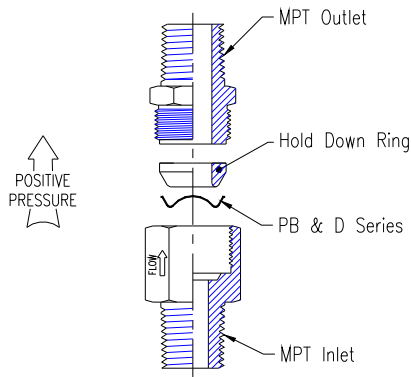
Figure 3 – Angle Seated Disk Screw Type Holder
