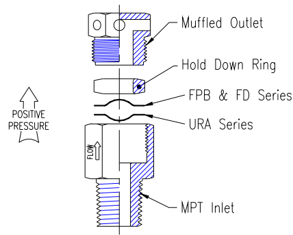
Figure 4 – Flat Seated Disk Screw Type Holder
